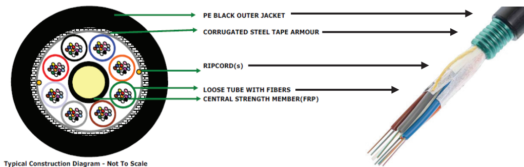
Figure 1 - An example of armor cable construction
