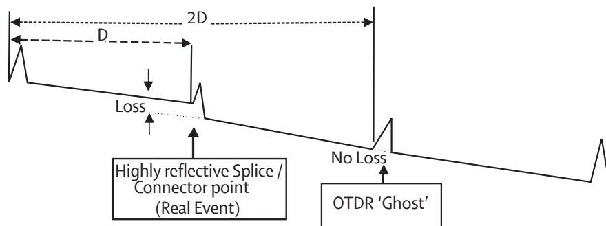
Fig. 2 OTDR real event and 'Ghost'
